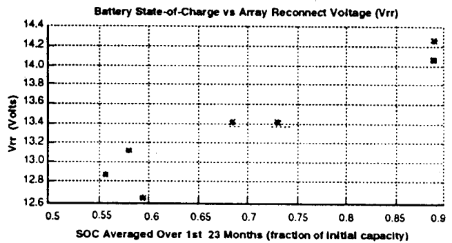
Figure 10: Average state-of-charge of the batteries at Sandia over the 23-month test as a function of regulation reconnect voltage (Vrr). Note that state-of-charge is strongly correlated to Vrr.
